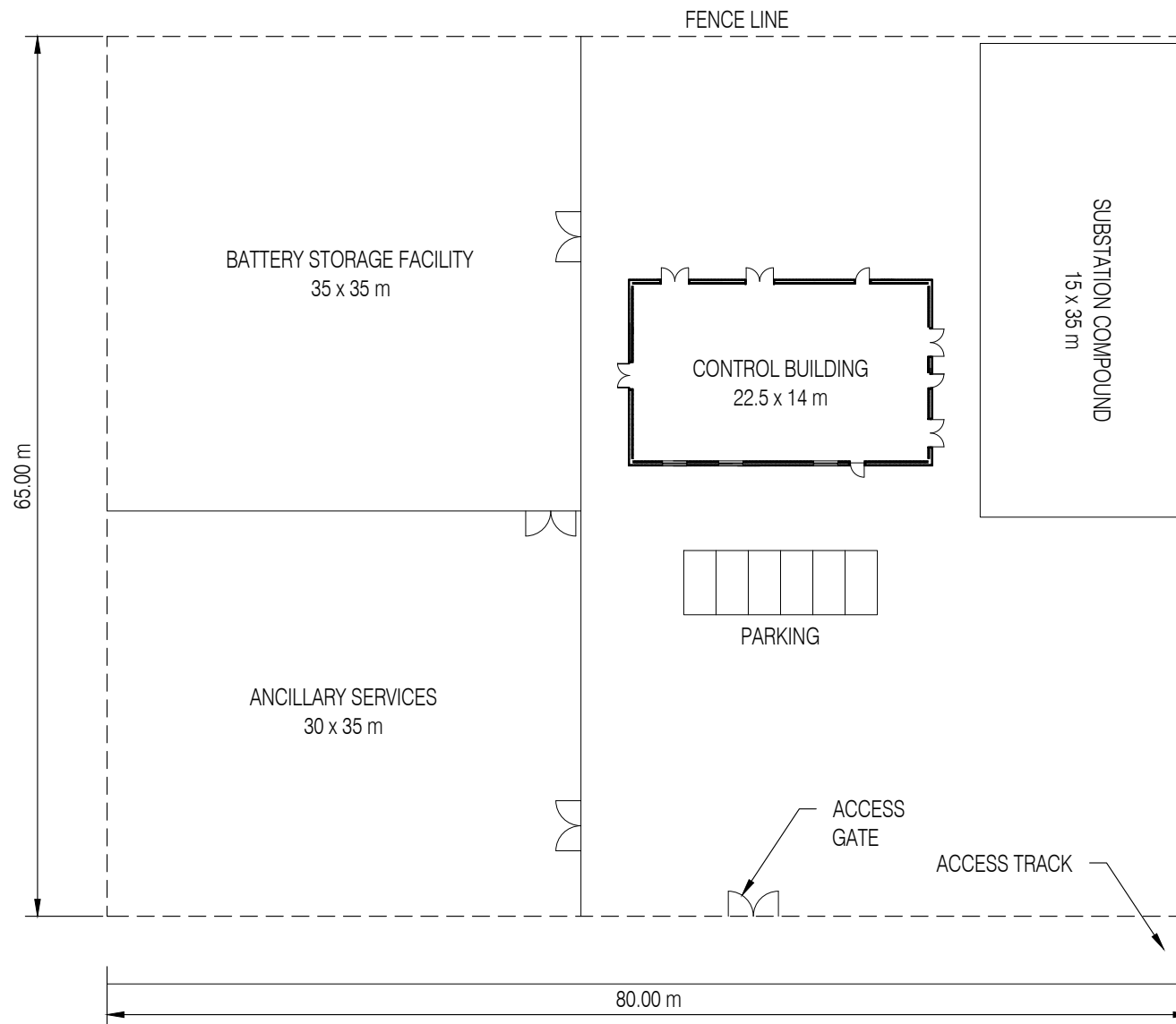
PLAN VIEW SCALE 1:500
